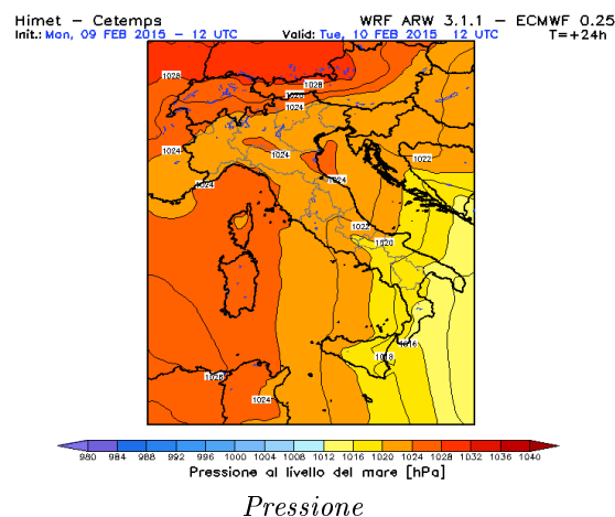
Himet - Cetemps WRF ARW 3.1.1 - ECMWF 0.25 Init.: Mon, 09 FEB 2015 - 12 UTC Valid: Tue, 10 FEB 2015 - 12 UTC T=+24h
