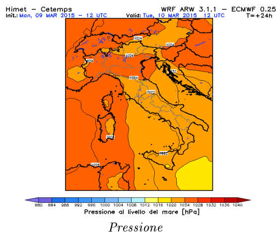
Himet - Cetemps WRF ARW 3.1.1 - ECMWF 0.25 Init.: Mon, 09 MAR 2015 - 12 UTC Valid: Tue, 10 MAR 2015 - 12 UTC T=+24h
