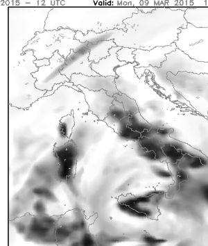
Himet - Cetemps WRF ARW 3.1.1 - ECMWF 0.25 Init.: Sun, 08 MAR 2015 - 12 UTC Valid: Mon, 09 MAR 2015, 12 UTC T=+24h
