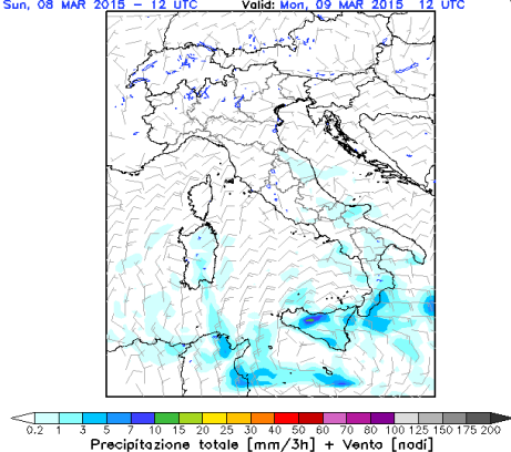
Himet - Cetemps WRF ARW 3.1.1 - ECMWF 0.25 Init.: Sun, 08 MAR 2015 - 12 UTC Valid: Mon, 09 MAR 2015, 12 UTC T=+24h
