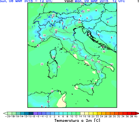
Himet - Cetemps WRF ARW 3.1.1 - ECMWF 0.25 Init.: Sun, 08 MAR 2015 - 12 UTC Valid: Mon, 09 MAR 2015, 12 UTC T=+24h
