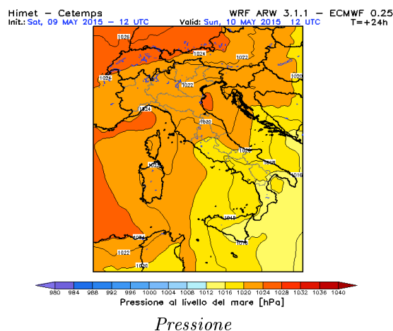
Himet - Cetemps WRF ARW 3.1.1 - ECMWF 0.25 Init.: Sat, 09 MAY 2015 - 12 UTC Valid: Sun, 10 MAY 2015 - 12 UTC T=+24h
