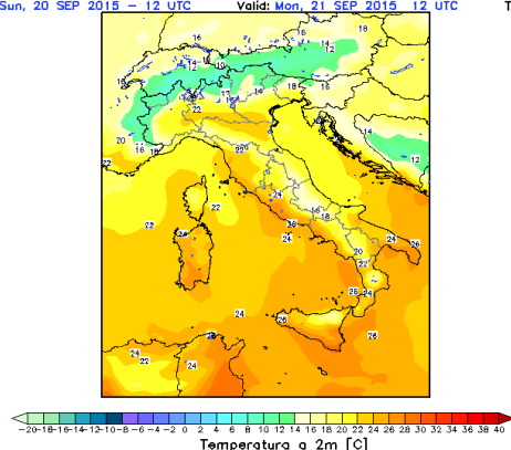
Himet - Cetemps WRF ARW 3.1.1 - ECMWF 0.25 Init.: Sun, 20 SEP 2015 - 12 UTC Valid: Mon, 21 SEP 2015, 12 UTC T=+24h
