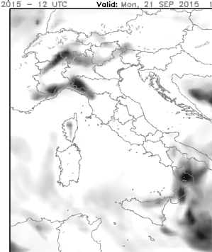
Himet - Cetemps WRF ARW 3.1.1 - ECMWF 0.25 Init.: Sun, 20 SEP 2015 - 12 UTC Valid: Mon, 21 SEP 2015, 12 UTC T=+24h
