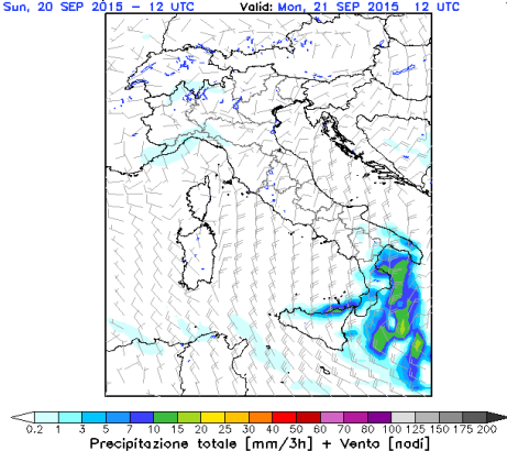
Himet - Cetemps WRF ARW 3.1.1 - ECMWF 0.25 Init.: Sun, 20 SEP 2015 - 12 UTC Valid: Mon, 21 SEP 2015, 12 UTC T=+24h
