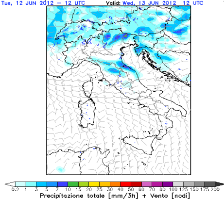
Himet - Cetemps WRF ARW 3.1.1 - ECMWF 0.25 Init.: Tue, 12 JUN 2012 - 12 UTC Valid: Wed, 13 JUN 2012 - 12 UTC T=+24h
