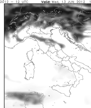
Himet - Cetemps WRF ARW 3.1.1 - ECMWF 0.25 Init.: Tue, 12 JUN 2012 - 12 UTC Valid: Wed, 13 JUN 2012 - 12 UTC T=+24h
