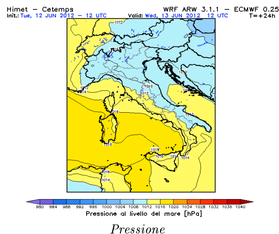
Himet - Cetemps WRF ARW 3.1.1 - ECMWF 0.25 Init.: Tue, 12 JUN 2012 - 12 UTC Valid: Wed, 13 JUN 2012 - 12 UTC T=+24h
