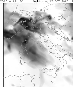
Himet - Cetemps Init.: Sun, 11 OCT 2015 - 12 UTC WRF ARW 3.1.1 - ECMWF 0.25 Valid: Mon, 12 OCT 2015, 12 UTC T=+24h
