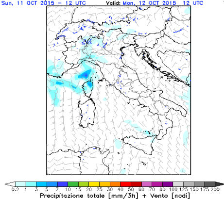
Himet - Cetemps Init.: Sun, 11 OCT 2015 - 12 UTC WRF ARW 3.1.1 - ECMWF 0.25 Valid: Mon, 12 OCT 2015, 12 UTC T=+24h
