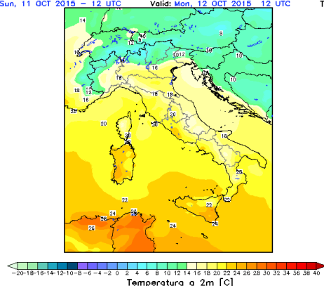
Himet - Cetemps Init.: Sun, 11 OCT 2015 - 12 UTC WRF ARW 3.1.1 - ECMWF 0.25 Valid: Mon, 12 OCT 2015, 12 UTC T=+24h
