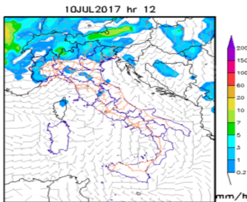
Arpa Lazio - prec - run 20170710 forecast +12h - WRF-ARW 3.5.1
