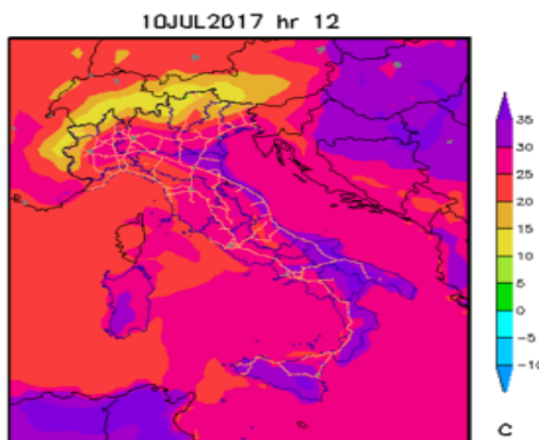
Arpa Lazio - t - run 20170710 forecast +12h - WRF-ARW 3.5.1
