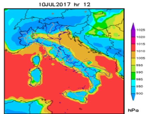
Arpa Lazio - p - run 20170710 forecast +12h - WRF-ARW 3.5.1
