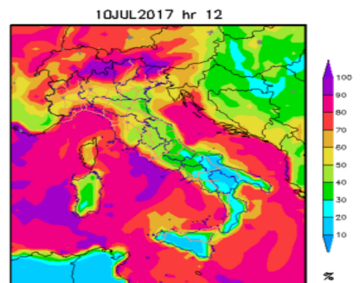
Arpa Lazio - rh - run 20170710 forecast +12h - WRF-ARW 3.5.1
