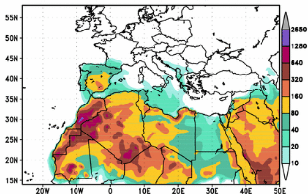
BSC-DREAM8b Lowest Model Level Dust Conc. ( \mu\text{g}/\text{m}^3 ) 24h forecast for 12UTC 09 AUG 12
