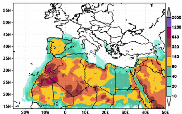
BSC-DREAM8b Lowest Model Level Dust Conc. ( \mu\text{g}/\text{m}^3 ) 48h forecast for 12UTC 10 AUG 12
