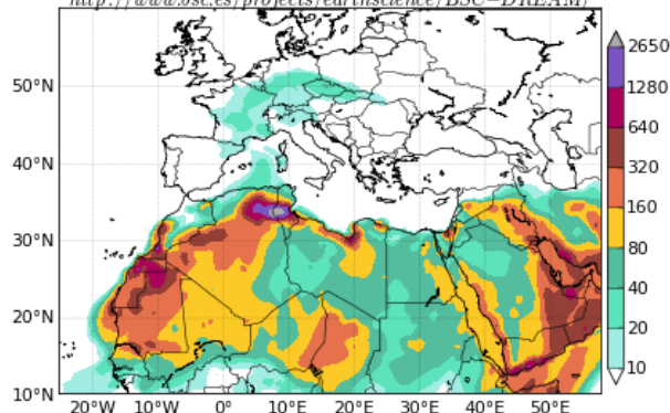
BSC-DREAM8b v2.0 Dust Low Level Conc. ( \mu\text{g}/\text{m}^3 ) 48h forecast for 12UTC 19 Jun 2013
