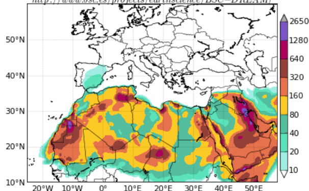
BSC-DREAM8b v2.0 Dust Low Level Conc. ( \mu\text{g}/\text{m}^3 ) 48h forecast for 12UTC 20 Jul 2013
