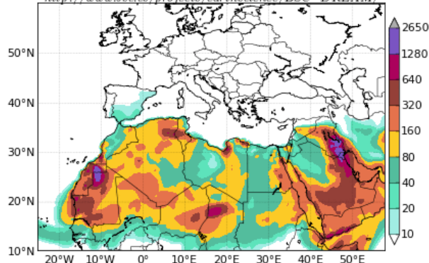
BSC-DREAM8b v2.0 Dust Low Level Conc. ( \mu\text{g}/\text{m}^3 ) 24h forecast for 12UTC 19 Jul 2013
