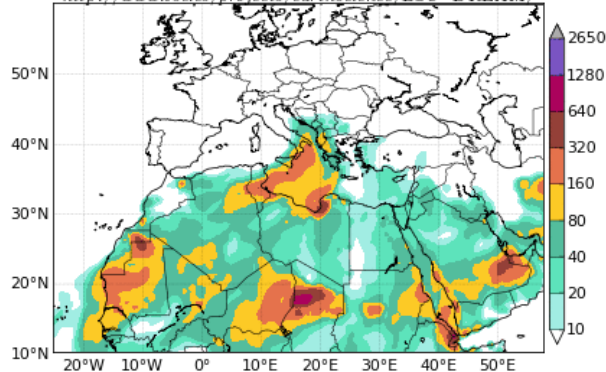
BSC-DREAM8b v2.0 Dust Low Level Conc. ( \mu\text{g}/\text{m}^3 ) 48h forecast for 12UTC 20 Nov 2013
