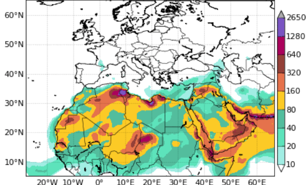
BSC-DREAM8b v2.0 Dust Low Level Conc. ( \mu\text{g}/\text{m}^3 ) 48h forecast for 12UTC 21 Apr 2016
