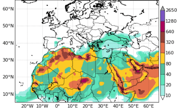
BSC-DREAM8b v2.0 Dust Low Level Conc. ( \mu\text{g}/\text{m}^3 ) 24h forecast for 12UTC 20 Apr 2016
